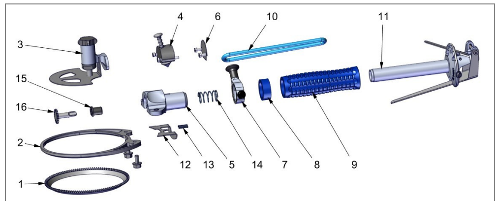
Fig. 3-1 Electric trimmer 128_evo3 (example)
