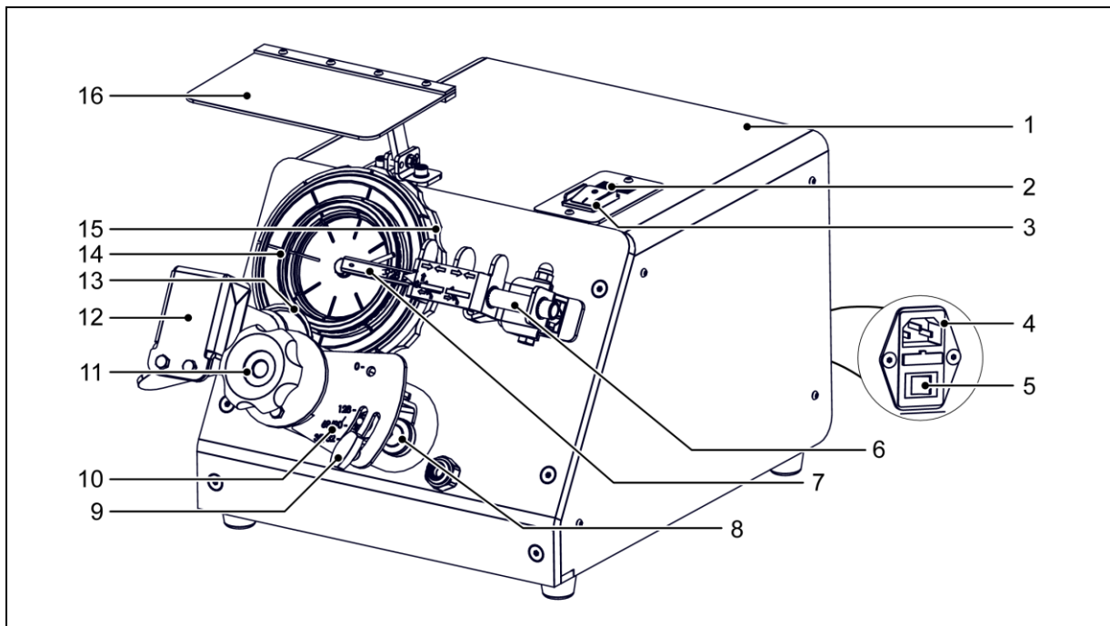
Fig. 3-8 View of TSM E1
