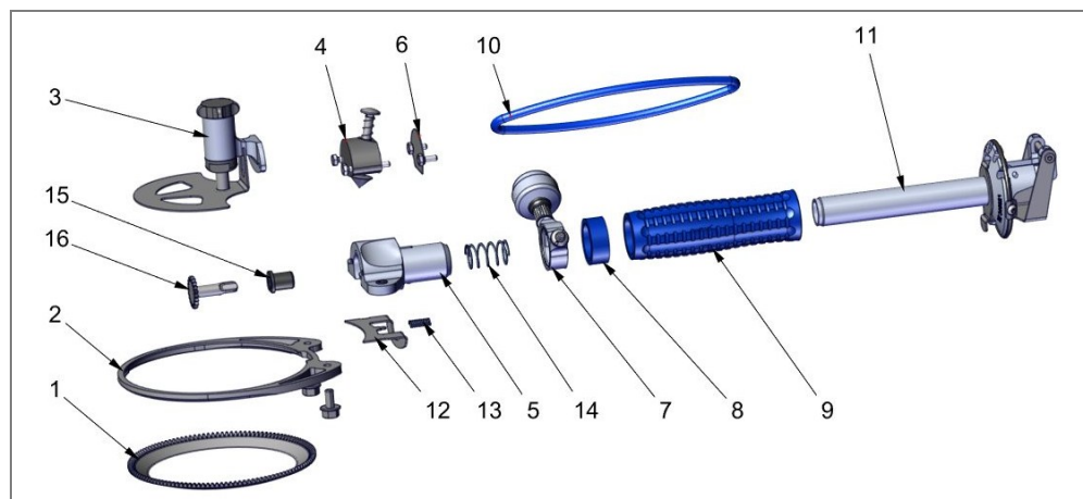
Fig. 3-2 Electric trimmer 128_evo3 (example)
