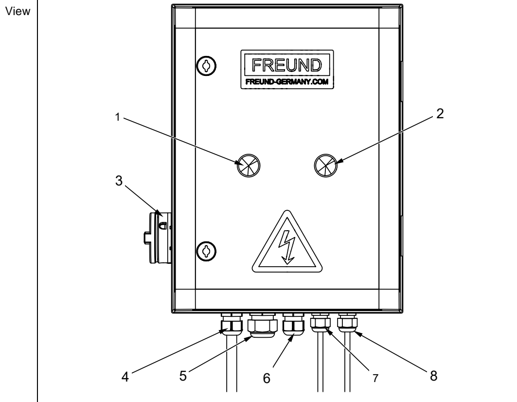
Fig. 3-9 View of control box SG WBS51-08
