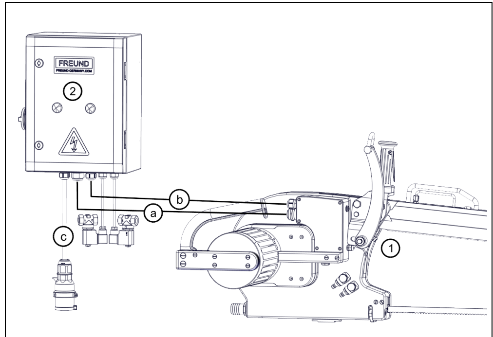
Fig. 5-6 Connection diagram
