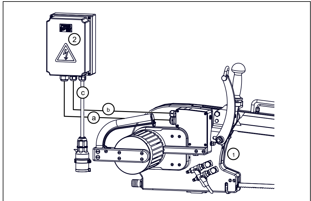
Fig. 5-8 Connection diagram
