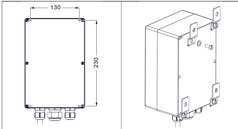
Fig. 5-4 Control box hole pattern SG WBS51-08nc [specifications in mm]
