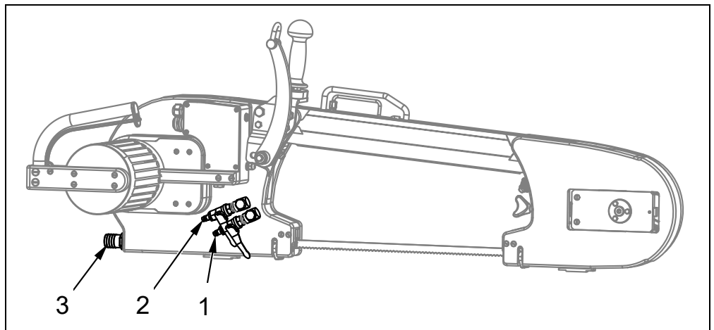
Fig. 5-9 Water connection
