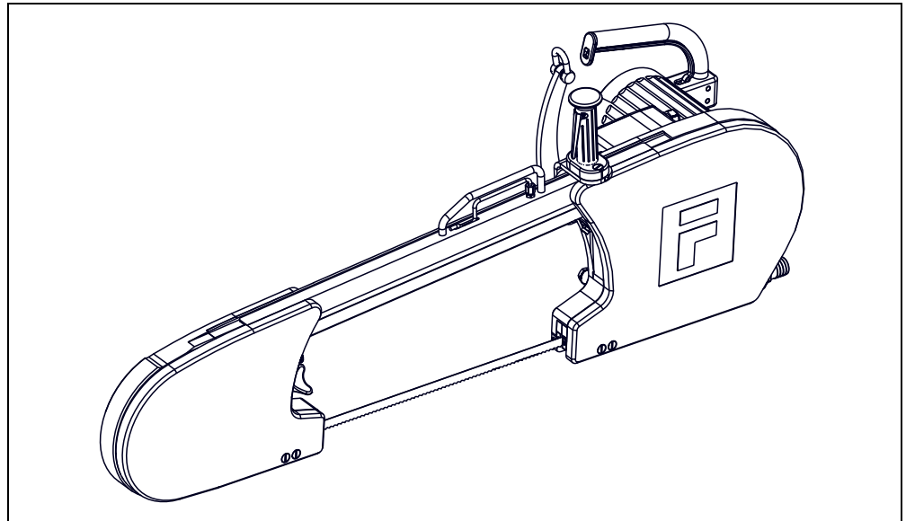
Fig. 3-1 view WBS51-08
