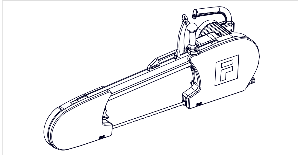
Fig. 3-5 view WBS51-08nc
