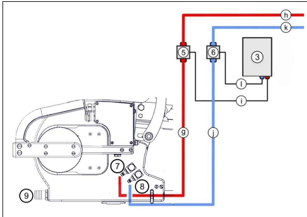
Fig. 5-7 Connection diagram
